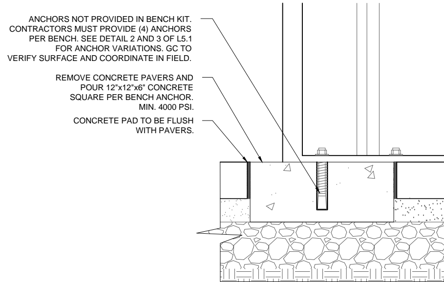
1 BENCH INSTALL: CONCRETE PAVER SCALE: 1-1/2"=1'
