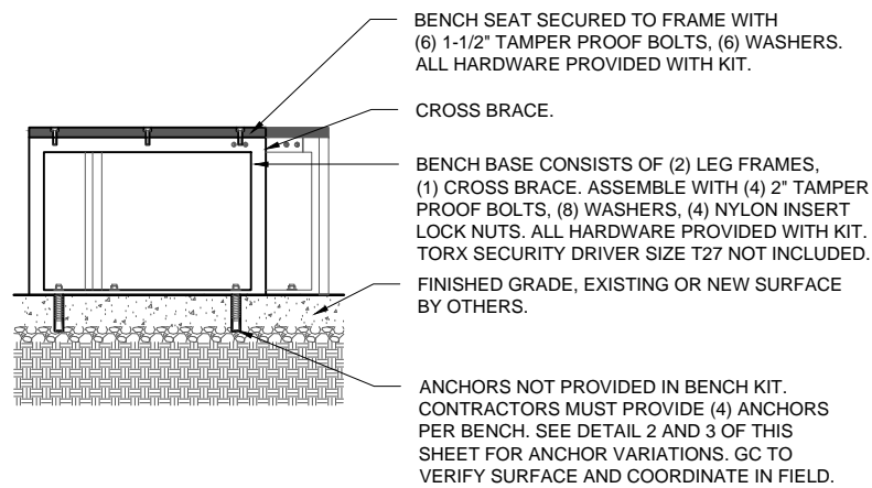
1 BENCH SCALE: 1/2"=1'
