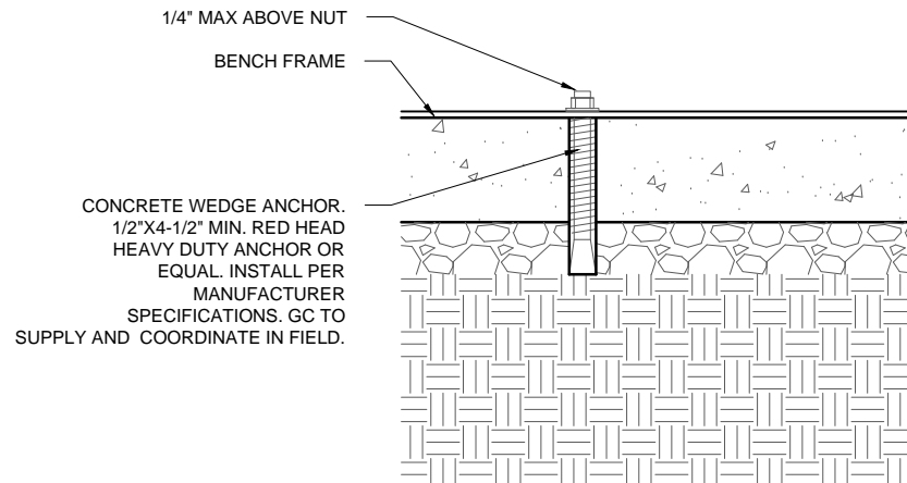
2 CONCRETE BENCH ANCHOR SCALE: 1-1/2"=1'
